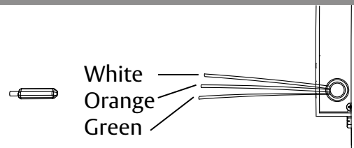
Diagram 1: Monitoring Switches
